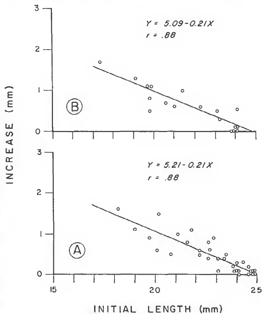
Figure 7. Growth of Littorina irrorata during 50 days at elevations 0.15 m (A) and 0.20 m (B).
